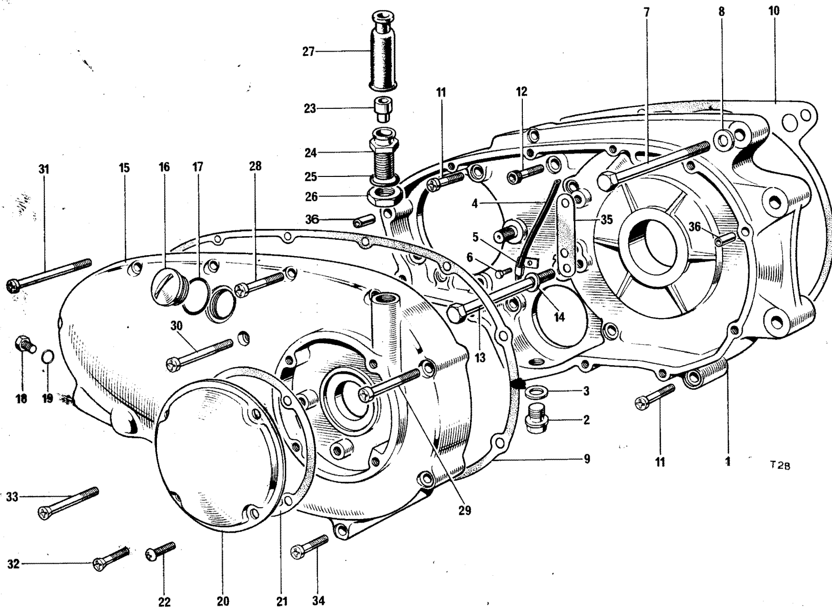
Fig. 12. INNER AND OUTER CHAINCASE
