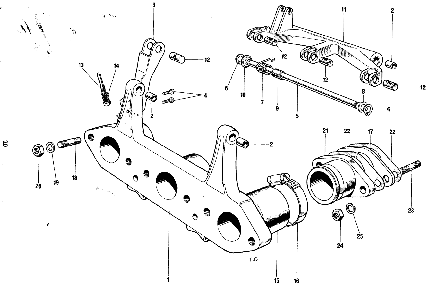
Fig. 7. MANIFOLD AND THROTTLE LINKAGE
