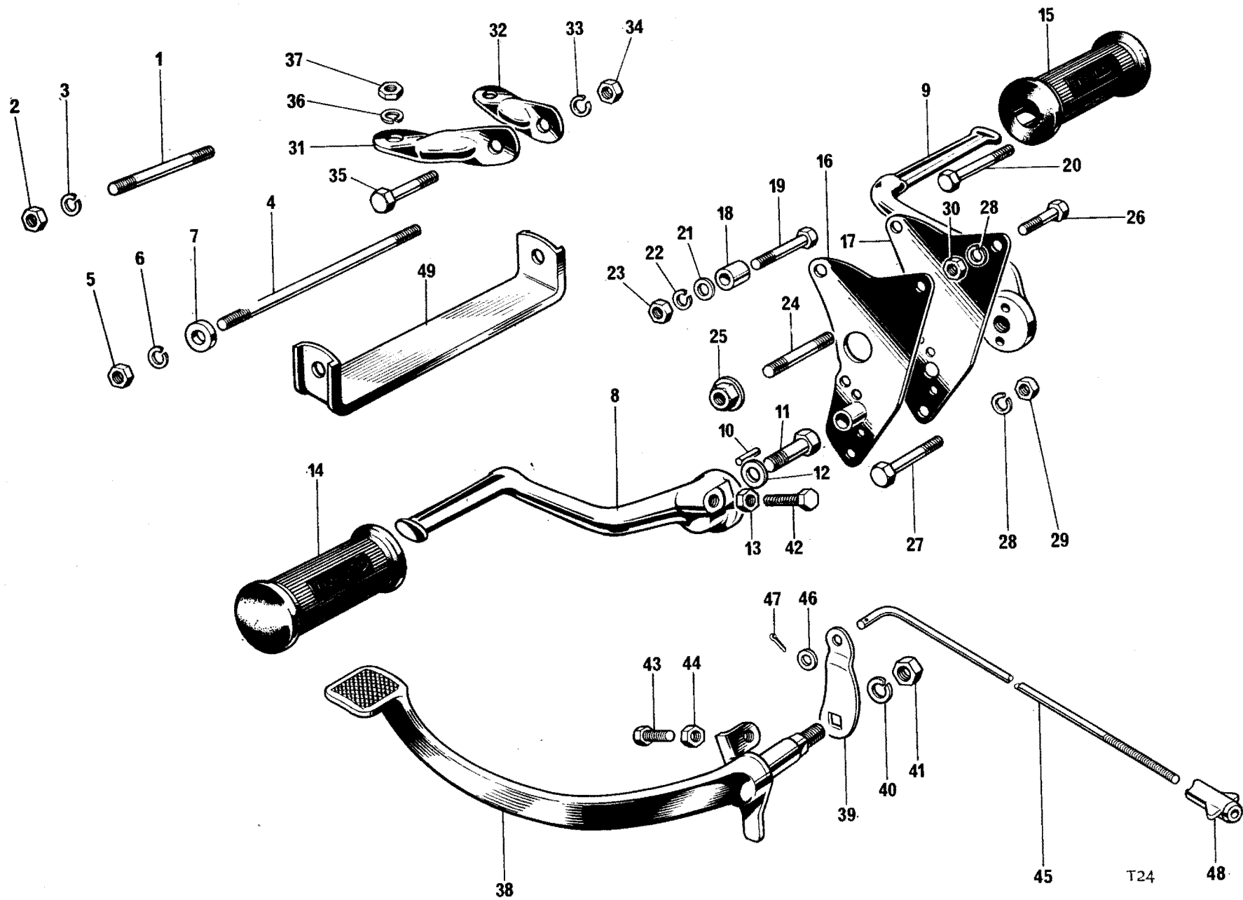
Fig. 16. ENGINE UNIT FITTINGS AND FOOTRESTS
