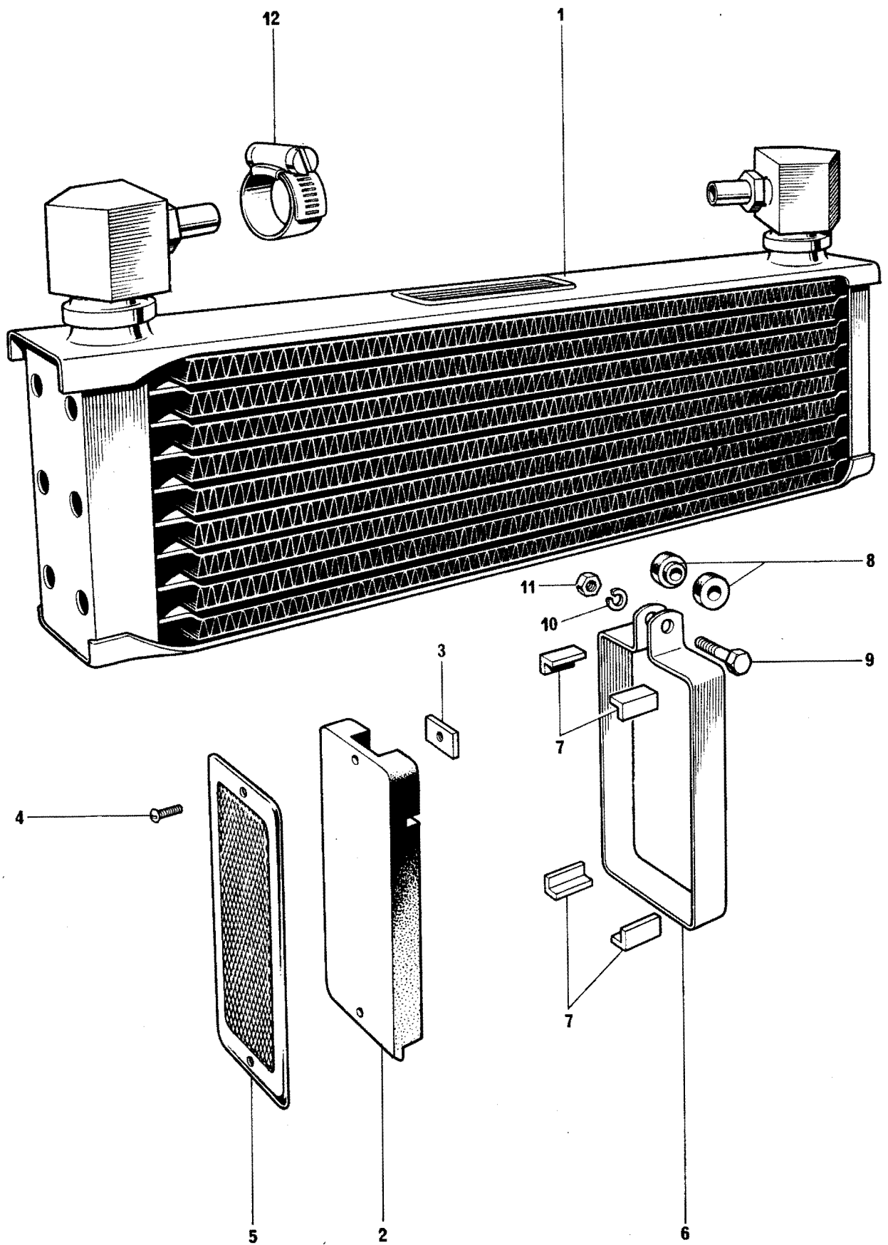
Fig. 23. OIL COOLER
