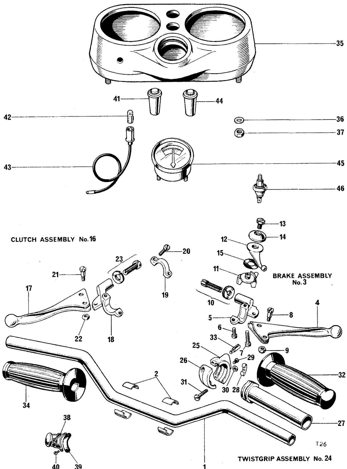
Fig. 30. HANDLEBARS, CONTROLS, BINNACLE AND OIL WARNING LIGHT
