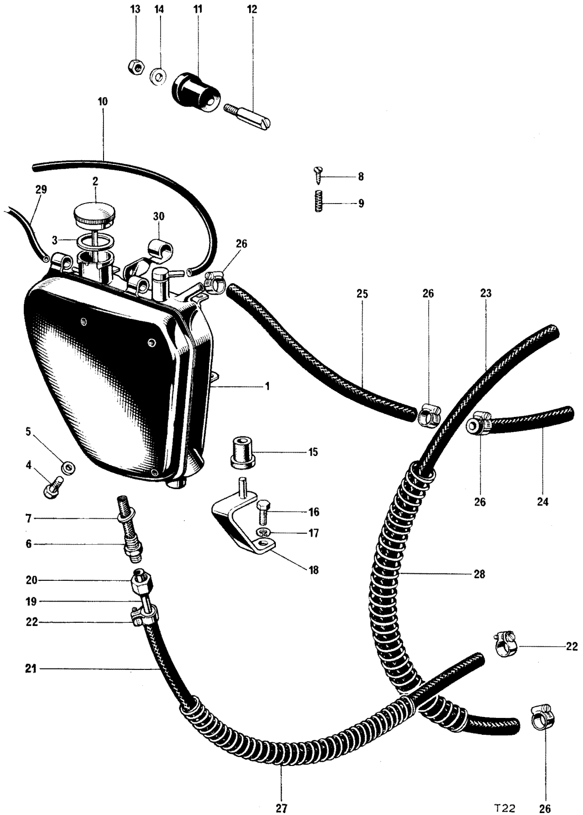
Fig. 25. OIL TANK
