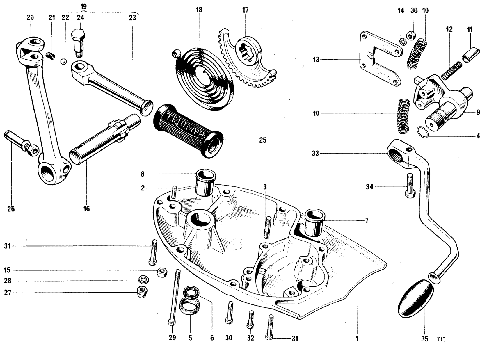
Fig. 8. GEARBOX OUTER COVER
